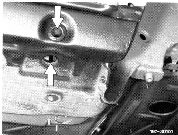
Vehicle jack tube, mount for plug (lifting platform) on floor laterally front and rear
